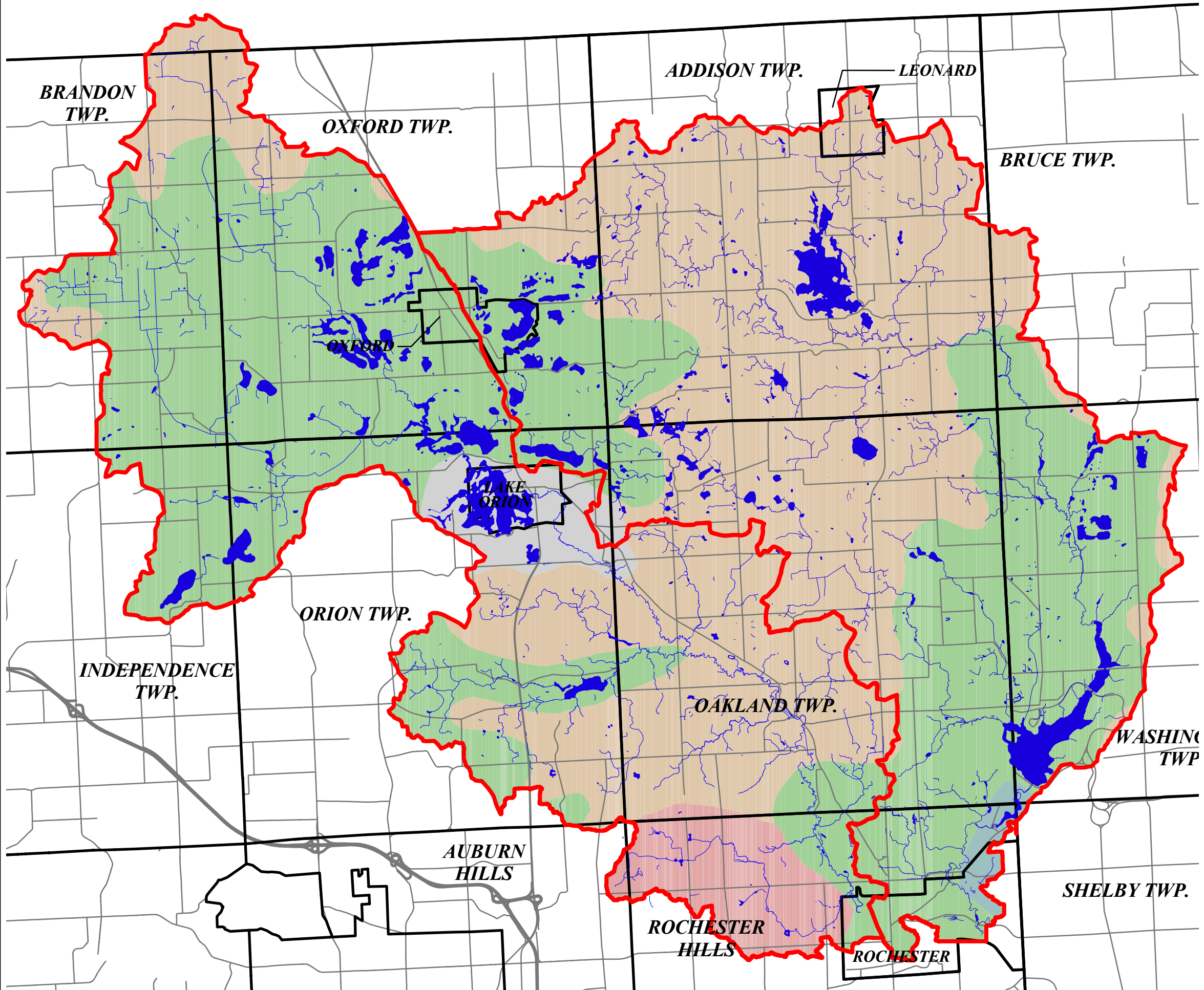
Figure 3.12. Generalized Soils
